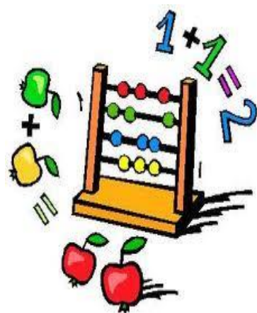
ARITHMETIC
